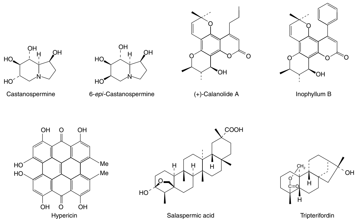
Fig. 30.2 Structures of potentially useful natural products for the treatment of AIDS. For other compounds see Table 30.2.
