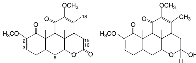
Quassin
