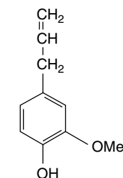
Eugenol
