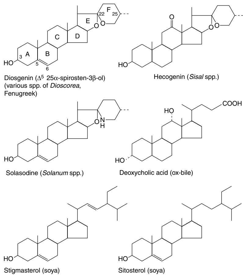
Fig. 23.5 Some naturally occurring steroids.
