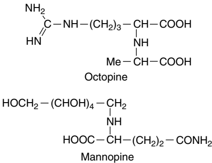
Fig. 14.3 Examples of opines.
