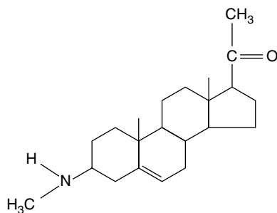
Holaphylline
