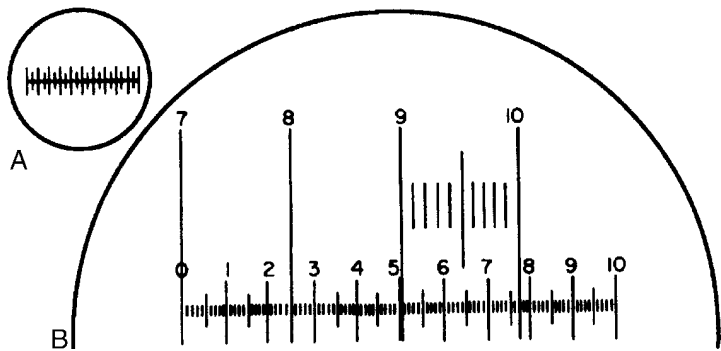
Fig. 43.1 A, Eyepiece micrometer; B, eyepiece micrometer superimposed on portion of stage micrometer scale.
