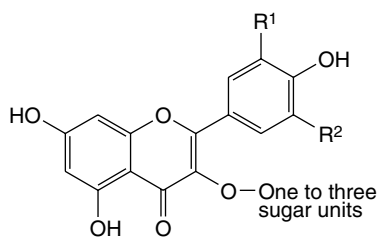
Flavonol structures
