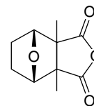
Cantharidin
