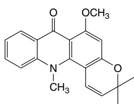
Acronycine
