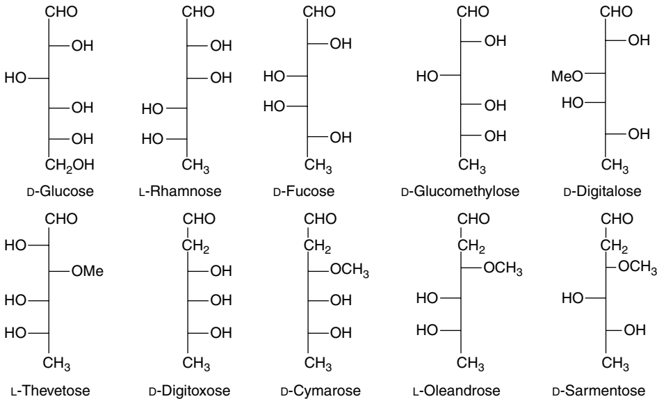
Fig. 23.15 Some examples of sugars found in cardiac glycosides (Fischer representation).
