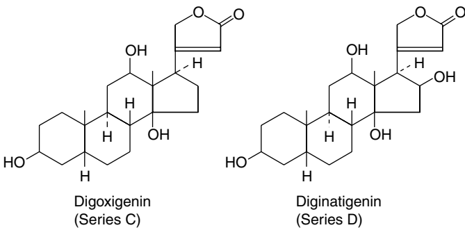
Fig. 23.20 Aglycones of Digitalis lanata cardioactive glycosides. See Fig. 23.19 for those also found in D. purpurea .
