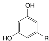
Cardanols
