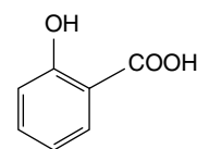
Salicylic acid
