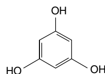
Phloroglucinol
