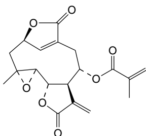
Elephantopin
