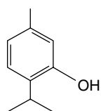
Thymol
