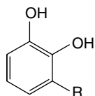
Urushiol phenols
