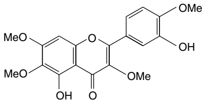
Casticin (Flavonoid)
